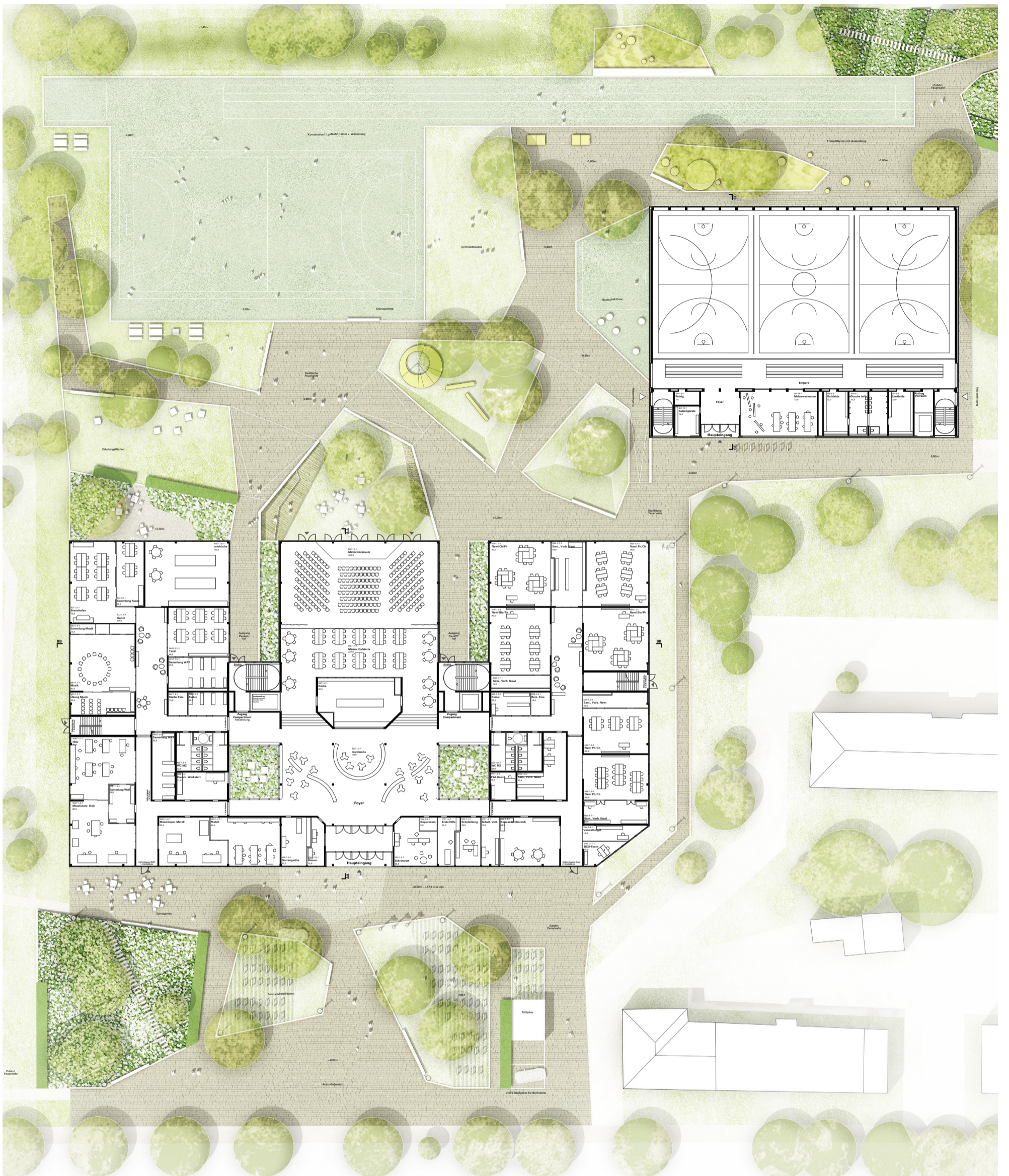
Grundriss Erdgeschoss 1_200
